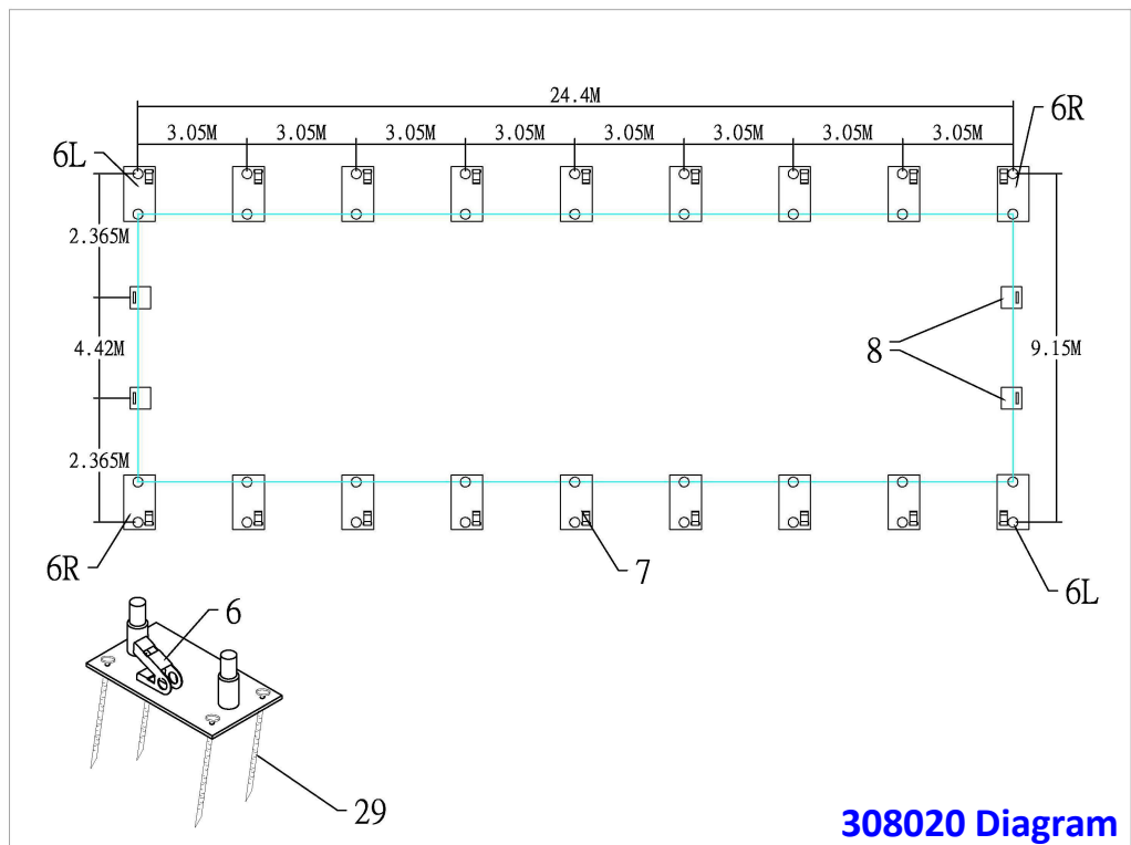
Figure 2: Foundation placement
